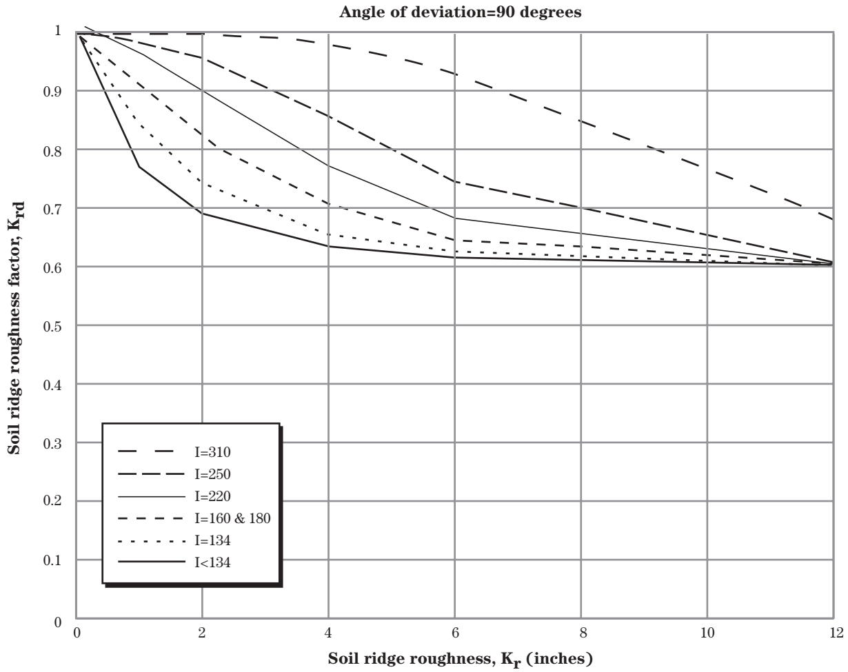
Exhibit 502-4 Ridge roughness factor, K_{rd} , graph—Continued
