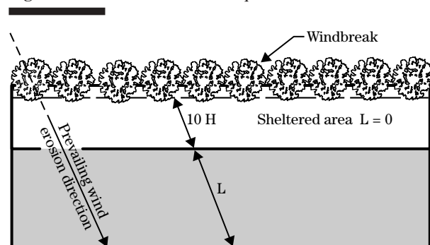
Figure 502-7 Unsheltered distance L – windbreak or barrier
