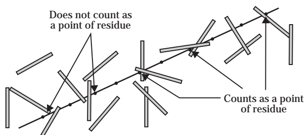
Figure 503-2 Counting residue pieces along a line transect
