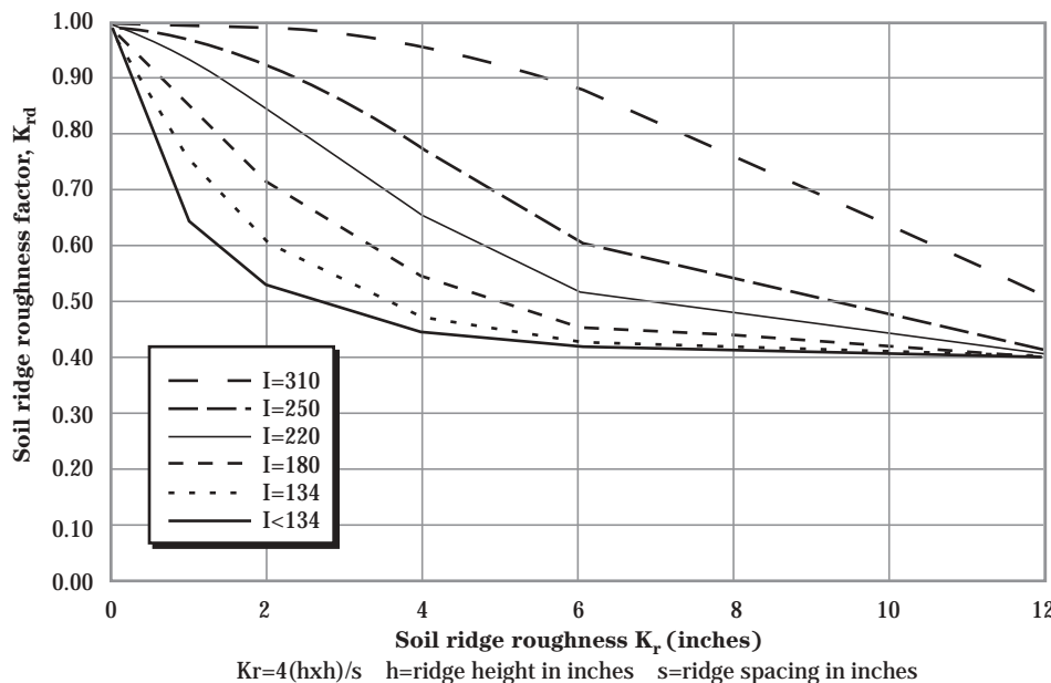
Figure 502-4 Chart to determine soil ridge roughness factor, K_{rd} , from ridge roughness, K_r , (inches). Only this chart, representing an angle of deviation of 0^\circ , will be used for the WEQ critical period procedure . When using the management period procedure , see exhibit 502-4 for graphs representing additional angles of deviation. Note: This graph represents erosive wind energy 60% parallel and 40% perpendicular to the prevailing erosive wind. —Hagen 1996
