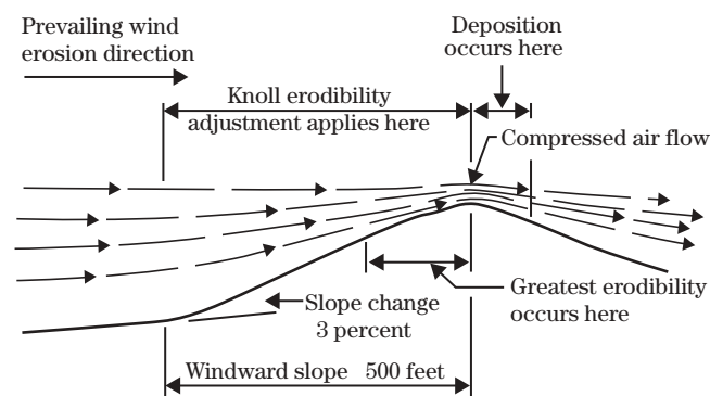
Figure 502-2 Graphic of knoll erodibility
