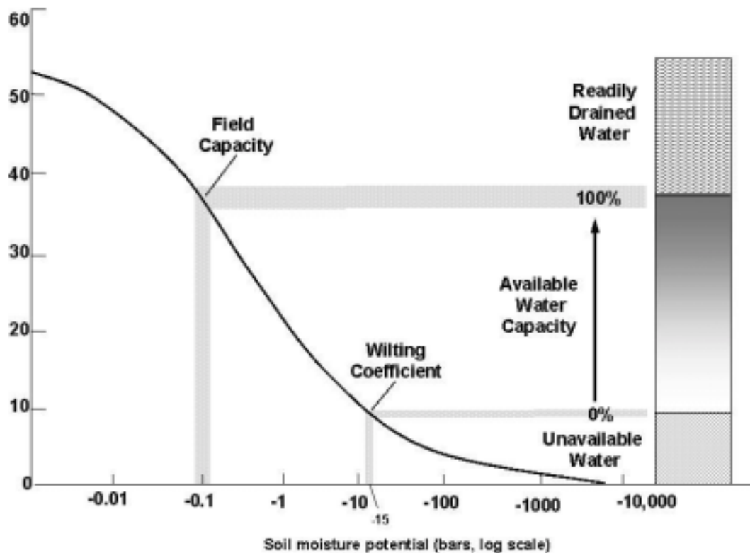
Figure 504-2 Relationship of soil moisture content and water availability to crops.
