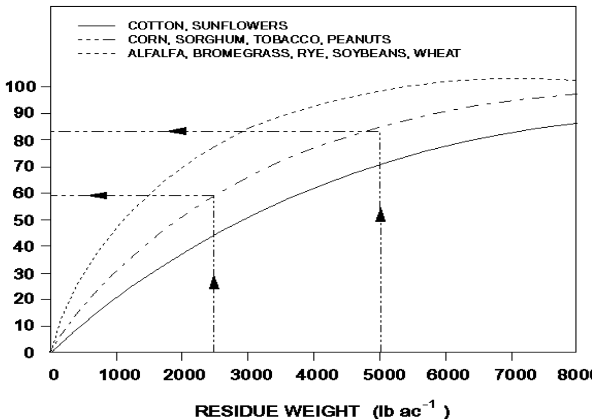
Figure 503-3 Relationship of residue weight to percent residue cover for various crops. Dashed lines with arrows illustrate the procedure to convert residue weight to percent residue cover.
