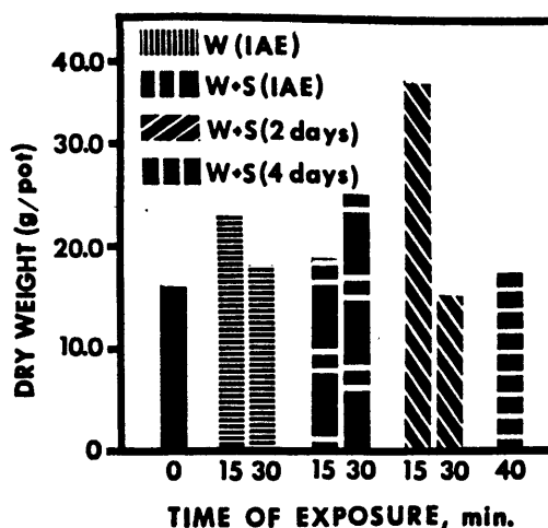
Fig. 2. Dry weight ( LSD_{05} = 3.0 g) of aerial portions of wheat plants exposed to varying degrees of mechanical injury and times of urea application.
