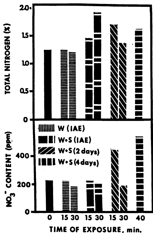
Fig. 1. Total nitrogen ( LSD_{05} = .31\% ) and nitrate ( LSD_{05} = 94 ppm) contents of aerial portions of wheat plants exposed to varying degrees of mechanical injury and times of urea application.
