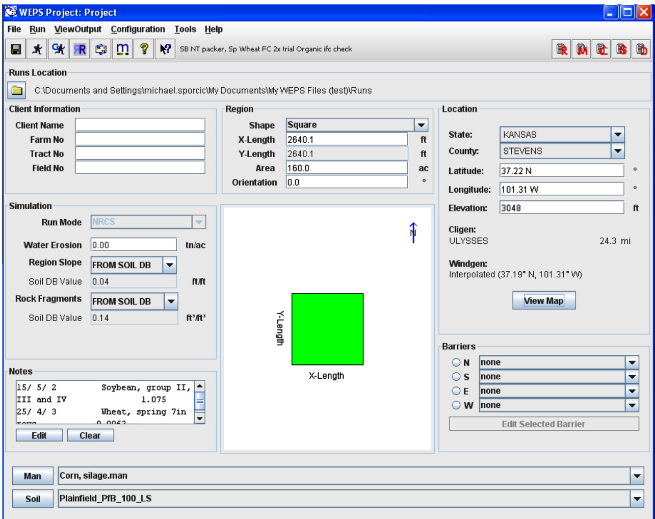
Fig. 3. Main screen of the WEPS user interface.
