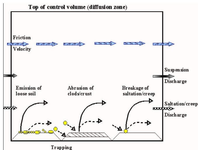
Figure 4. Diagram illustrating processes simulated by the EROSION submodel on a bare soil surface in an individual grid cell.
