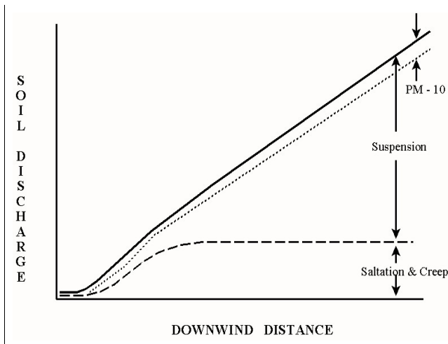
Figure 5. Diagram illustrating downwind transport capacity for saltation & creep, but a continuing increase in transported mass of suspension-size soil downwind.
