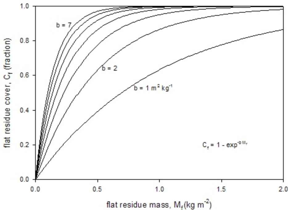
Figure 5.43. Relationship between flat residue mass and the cover provided by this flat residue.
