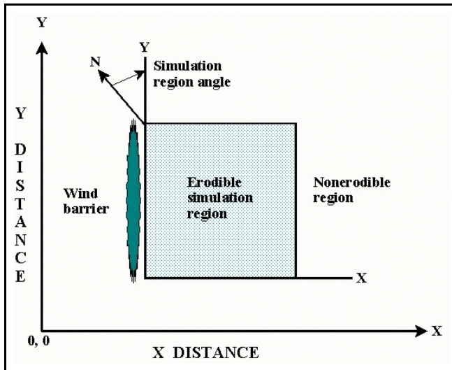
Figure 4.3. Schematic of simulation region geometry. Field orientation, end points of barriers, and opposite corners of the rectangular simulation region are input to the EROSION submodel.
