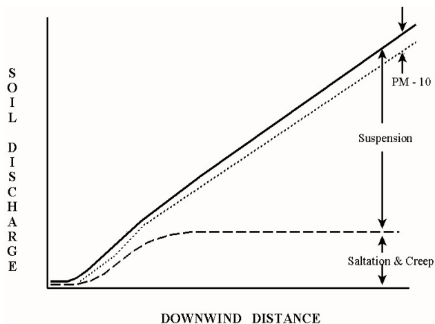
Figure 4.7. Diagram illustrating downwind transport capacity for saltation & creep, but a continuing increase in transported mass of suspension-size soil downwind.
