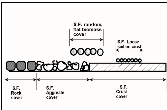
Figure 4.4. Diagram illustrating components of flat surface cover inputs to the EROSION submodel.
