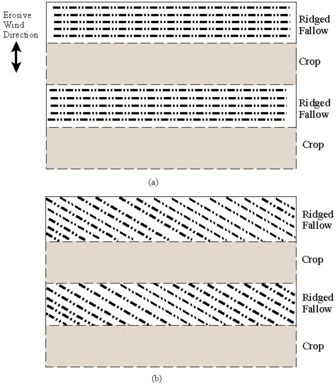
Figure 5.15. Designs using (a) parallel tillage ridges and (b) angled tillage ridges.
