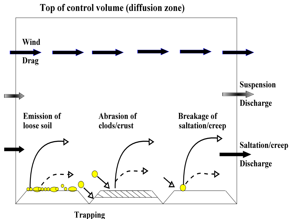
Figure 5.9. Wind erosion processes on a bare field simulated in WEPS.
