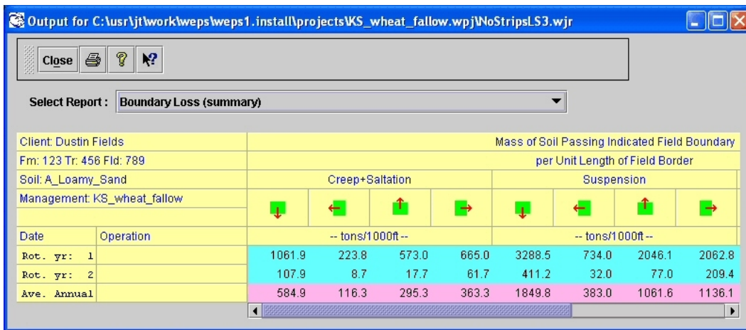
Figure 5.30. Boundary Loss summary for the non-stripped field with a loamy sand soil.
