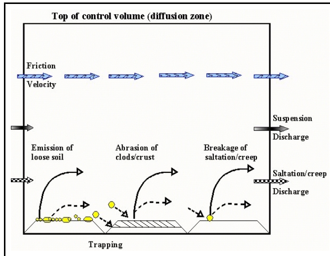
Figure 4.6. Diagram illustrating processes simulated by the EROSION submodel on a bare soil surface in an individual grid cell.
