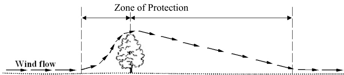
Figure 5.1. Diagram showing wind flow pattern over a barrier.
