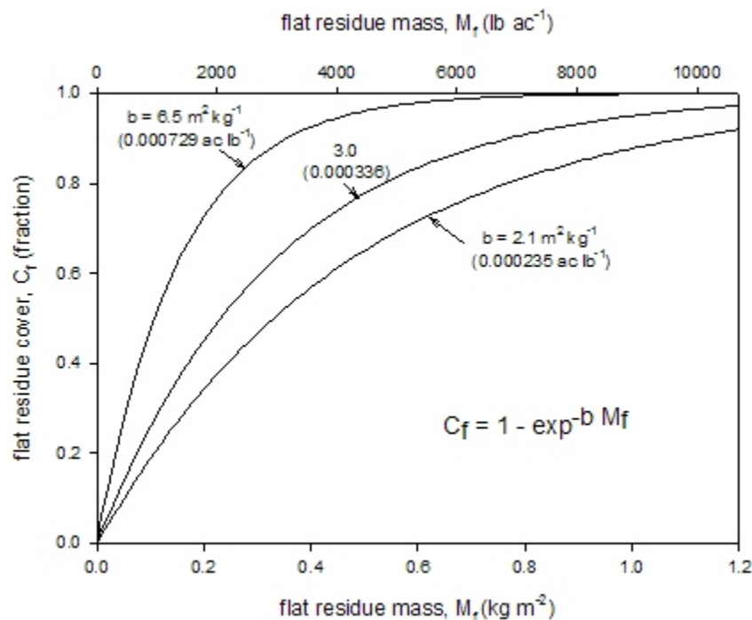
Figure 5.40. Relationship between flat residue mass and the cover provided by this flat residue for three different values of the mass-to-cover factor b . WEPS uses b = 6.5 \text{ m}^2 \text{ kg}^{-1} for wheat, barley, oats, rye, and triticale; b = 3.0 \text{ m}^2 \text{ kg}^{-1} for corn, sorghum, and millet; and b = 2.1 \text{ m}^2 \text{ kg}^{-1} for cotton and sunflower.
