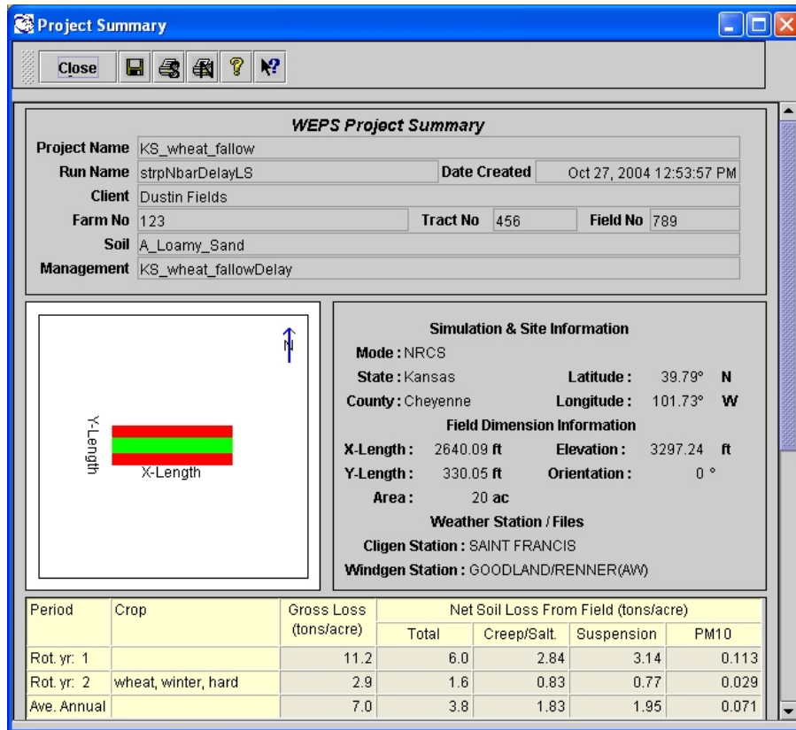
Figure 5.33. Run Summary for the strip-cropped field with barriers and a stubble mulch management system.
