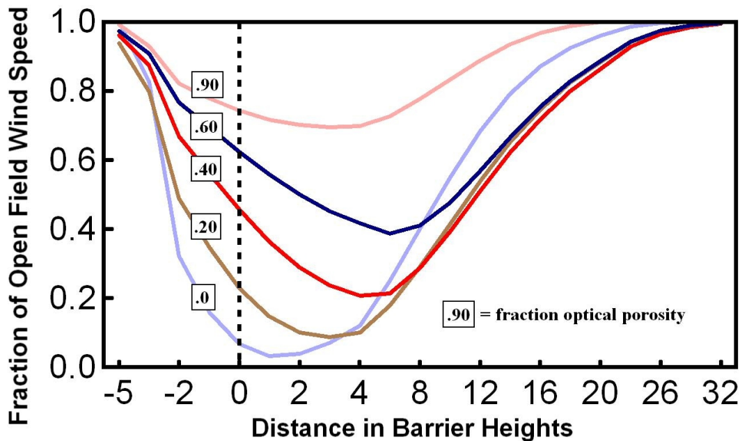
Figure 5.6. Effect of the fraction of optical porosity on near-surface wind speed along the wind direction relative to barrier. The “Distance in Barrier Heights” refers to the distance from the barrier at 0, measured in multiples of the barrier height.
