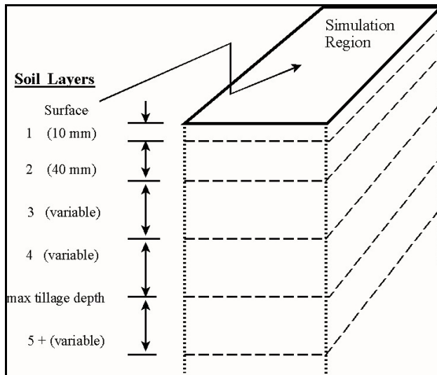
Figure 4.2. Diagram representing the spatial domain of the SOIL submodel.
