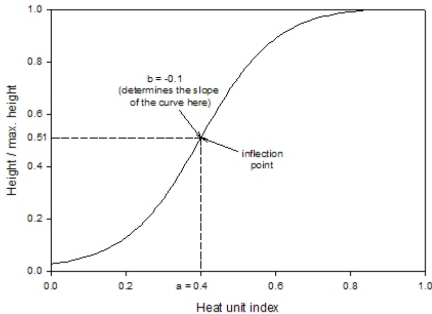
Figure 5.38. Crop height development function as it would be without any stresses. In this example, a = 0.4 and b = -0.1 . The height ratio at the inflection point = 0.51.
