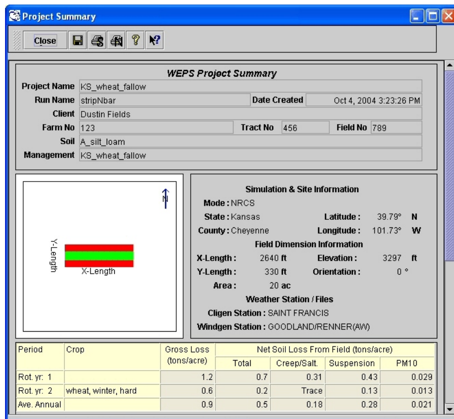
Figure 5.27. Run Summary report for the strip-cropped field with barriers.
