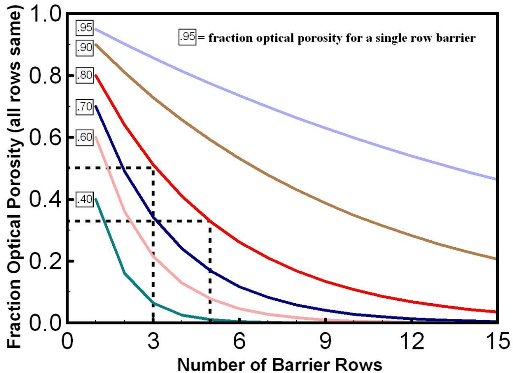
Figure 5.7. Effect of number of barrier rows on optical porosity when all barrier rows are the same.
