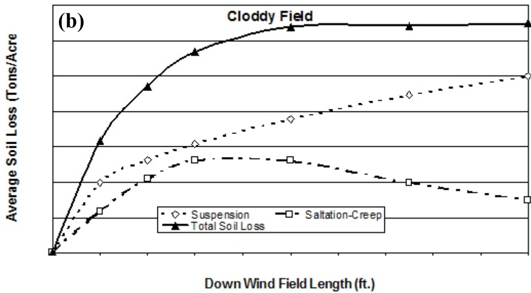
Figure 5.12. Comparison of average soil loss at various downwind distances on (a) a smooth, loose field and (b) a cloddy field.
