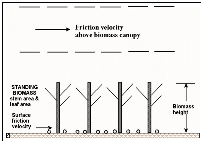
Figure 4.5. Diagram illustrating friction velocity above standing biomass that is reduced by drag of stems and leaves to the surface friction velocity below the standing biomass.
