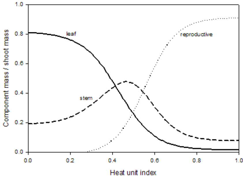
Figure 6.36. Partitioning of shoot mass (above-ground biomass) into component mass for winter wheat. Components are leaf, stem, and reproductive mass. By definition, these three fractions always add to 1.0.
