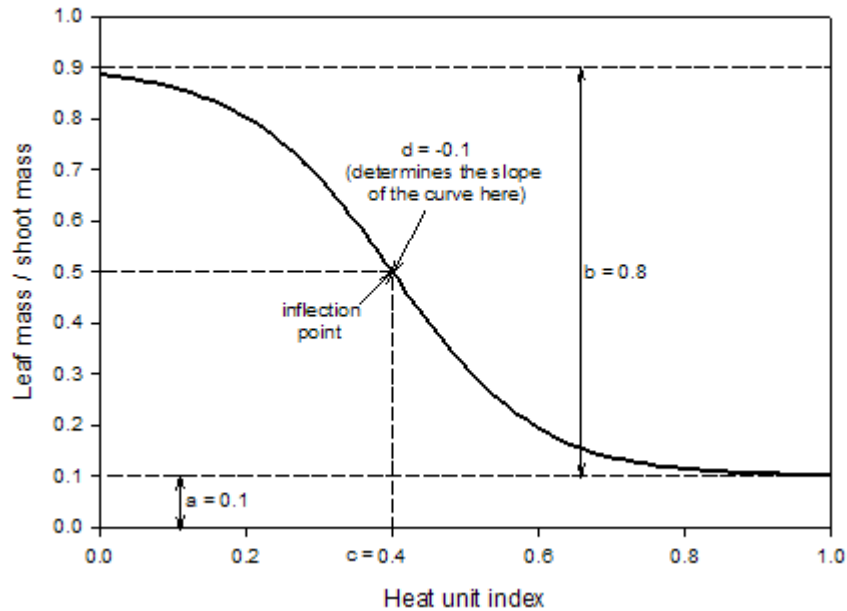
Figure 6.37. Partitioning of shoot mass into leaf mass. In this example, a = 0.1 , b = 0.8 , c = 0.4 , and d = -0.1 . The leaf mass / shoot mass ratio at the inflection point = a + b/2 = 0.5 .
